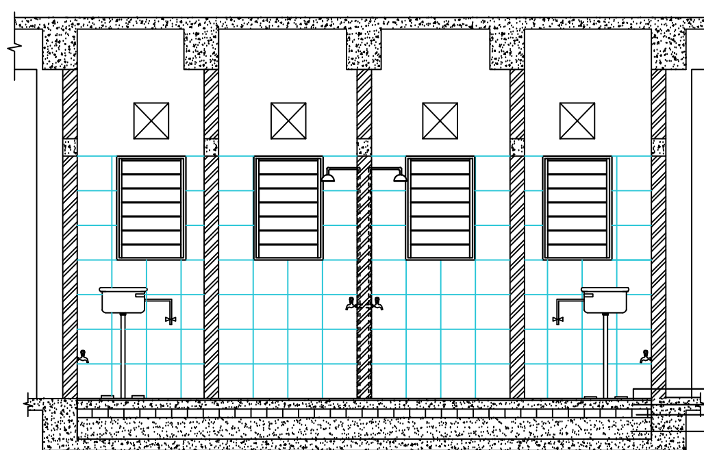
SECTION C-C
